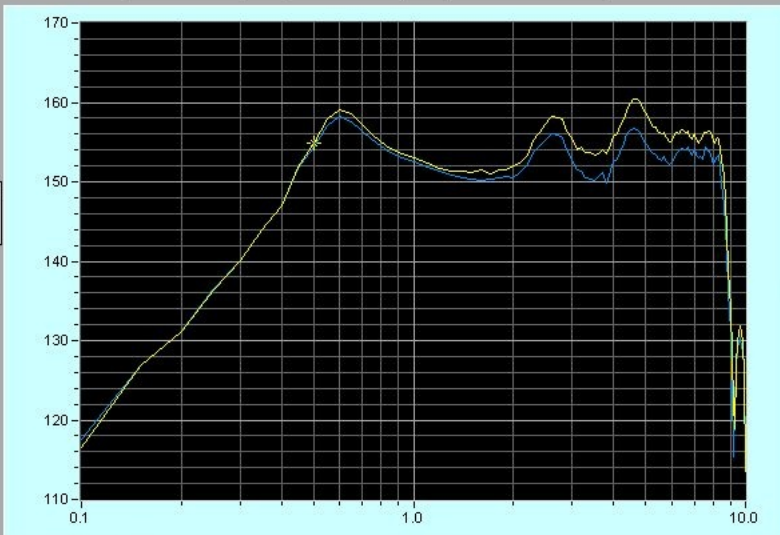
Transmit voltage response vs Frequency
