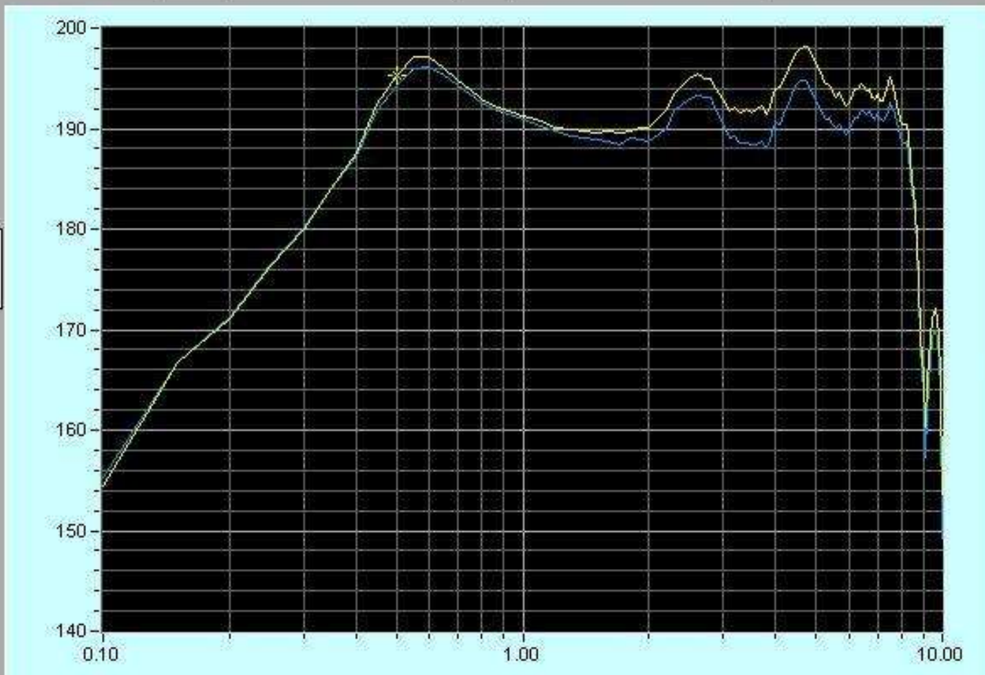
Sound pressure level vs Frequency
